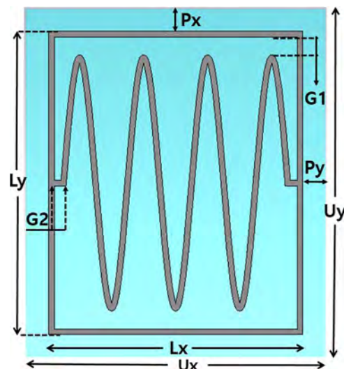
FIG. 2. Schematic view of the rectangular ring unit cell with the sinusoidal modulation index as 3.5 ( Lx = 13.6 , Ly = 16.2 , Ux = 14 , Uy = 16.6 , Px = 0.2 , Py = 0.2 , G1 = 1 , and G2 = 0.5 ) (all units in mm).
